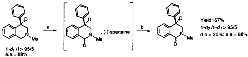
Scheme 2. (a) s -BuLi–(–)-sparteine/Et 2 O, 4 equiv./–78°C; (b) MeOD/–78°C
