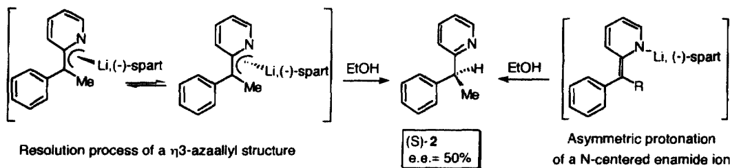
Scheme 3. Possible pathways of asymmetric induction during the deracemization of 2
